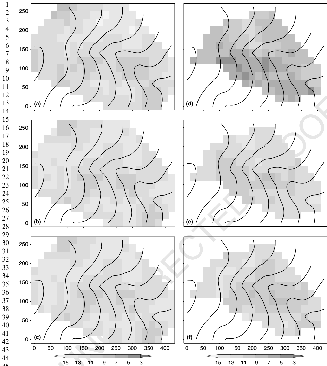
Figure 8. Predicted backscattering for Julian day 265 using inverted RMS surface roughness from Julian day 249 with: measured soil moisture and (a) IEM, (b) EM and (c) SEM backscattering models; modelled soil moisture and (d) IEM, (e) EM and (f) SEM backscattering models (dB). Contour lines are elevation with an interval of 5 m
