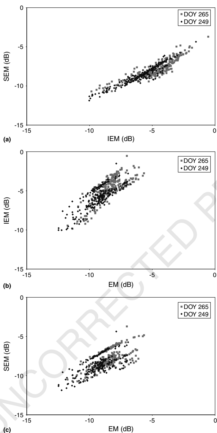
47 Figure 6. Comparison of the three backscattering model predictions with the same input data for soil moisture, soil properties and surface 48 roughness for Julian days 249 and 265 49
