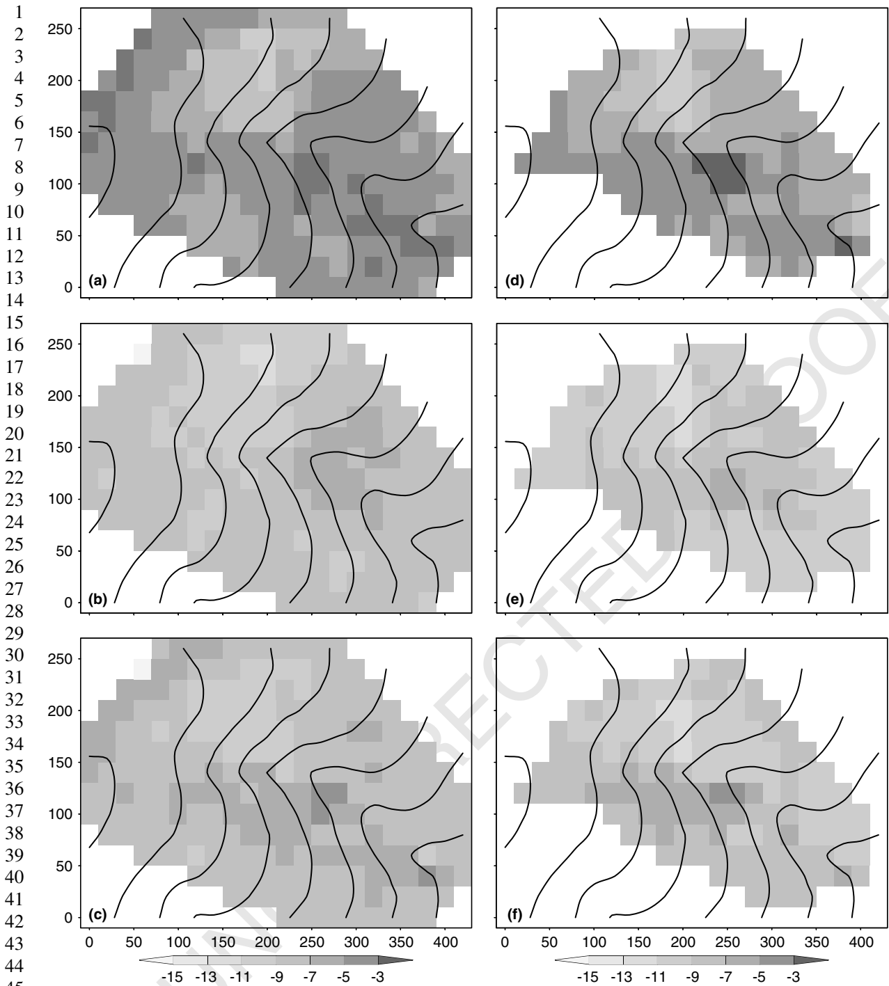
Figure 7. Predicted backscattering for Julian day 265 using measured RMS surface roughness with: measured soil moisture and (a) IEM, (b) EM and (c) SEM backscattering models; modelled soil moisture and (d) IEM, (e) EM and (f) SEM backscattering models (dB). Contour lines are elevation with an interval of 5 m
