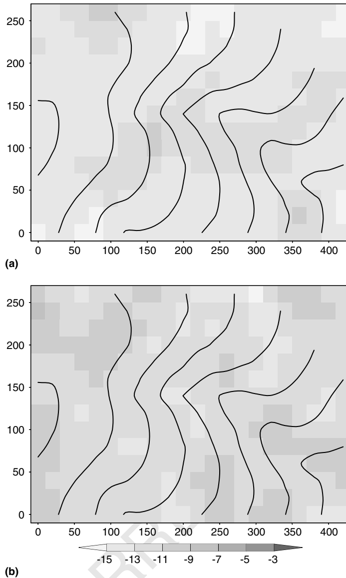
38 Figure 1. ERS-2 backscattering data (dB) on Julian day of year (a) 249 and (b) 265 after applying a 3 \times 3 filter. Contour lines are elevation 39 with an interval of 5 m
