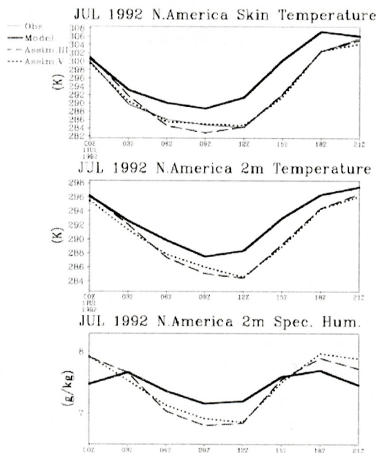
Figure 6. The July 1992 monthly mean diurnal cycle of skin temperature (top), 2 m temperature (middle) and 2 m specific humidity (bottom) over North America for the observations (light solid), Model (heavy solid), Assimilation III (dashed) and Assimilation V (dotted).
