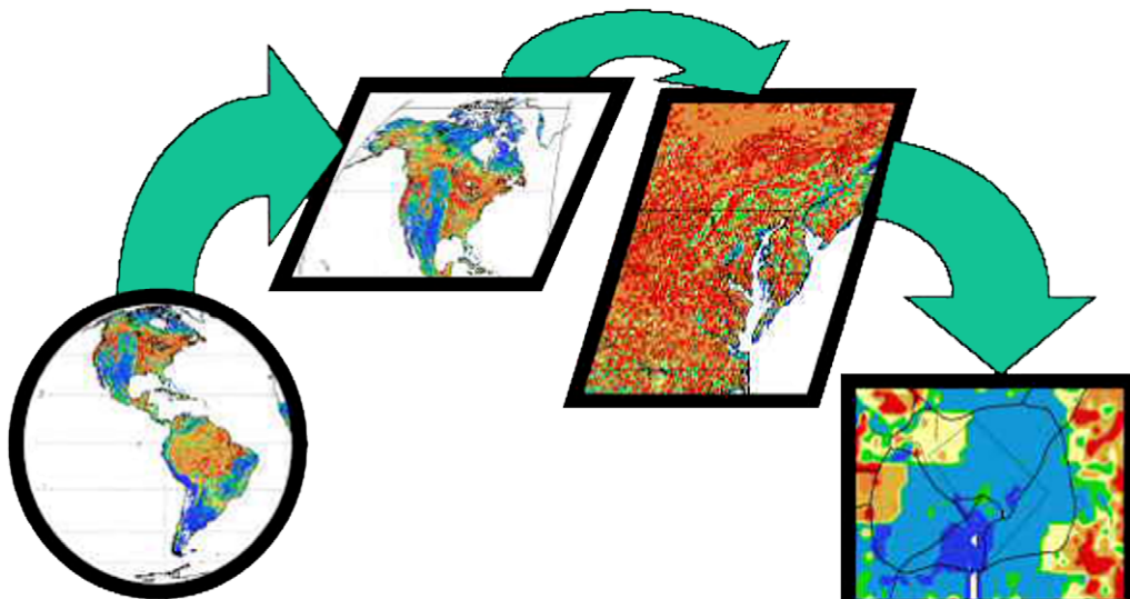
Fig. 3. One kilometer resolution global MODIS Leaf Area Index product.
