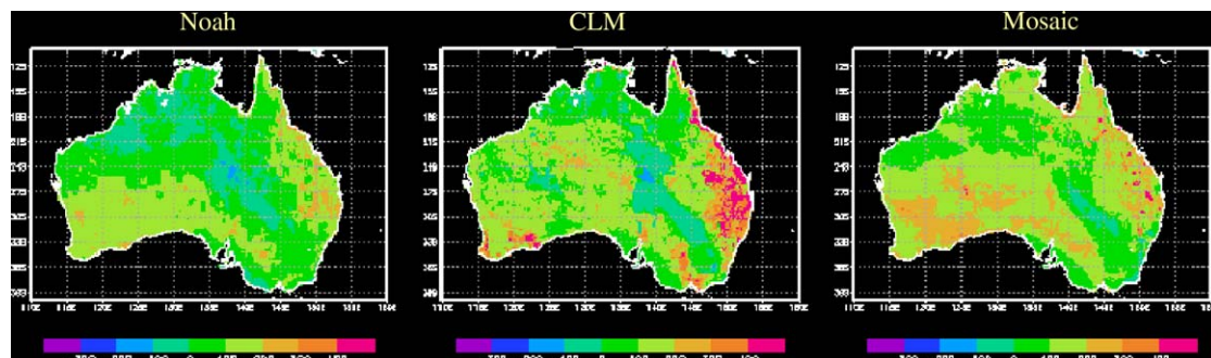
Fig. 8. Sensible heat fluxes ( \text{W/m}^2 ) produced by Noah, CLM, and Mosaic over Australia, at 4GMT for October 9, 2001.
