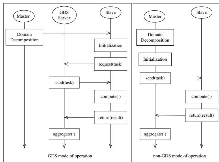
Fig. 4. Roles of master, slave, and the GDS server in different parallel modes of operation in LIS.
