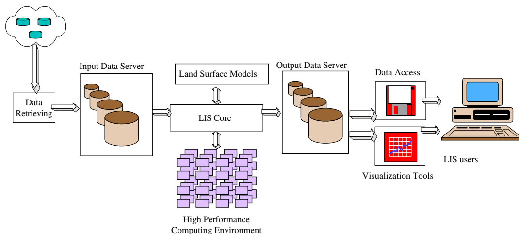
Fig. 2. Components of the LIS software architecture.
