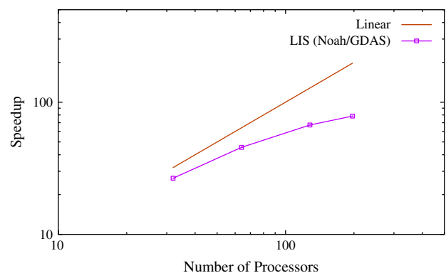
Fig. 14. Performance speedup vs number of processors for a global 1 km LIS simulation with Noah using the GDAS forcing compared with the theoretical linear scaling estimate.
