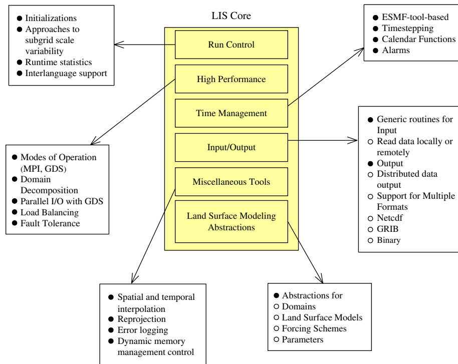
Fig. 6. Main functions of the LIS core.
