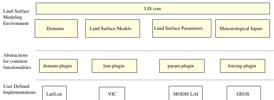
Fig. 5. Layered architecture of the LIS components.
