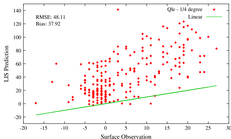
Fig. 11. Comparison of the latent heat fluxes from CLM at 25 km resolution with the surface observations at Fort Peck, MT, for the EOP-1 period.
