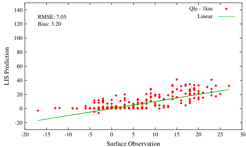
Fig. 12. Comparison of the latent heat fluxes from CLM at 1 km resolution with the surface observations at Fort Peck, MT, for the EOP-1 period.
