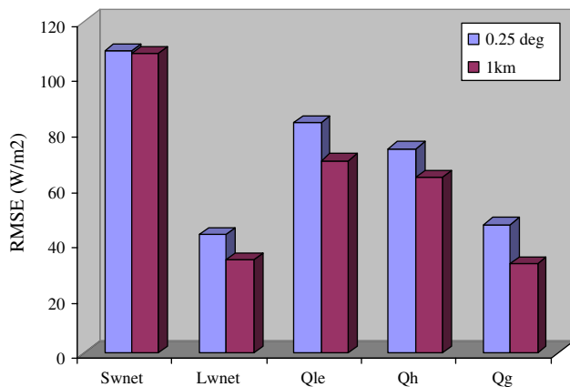
Fig. 13. Comparison of root mean square errors (RMSE) at 25 km and 1 km resolution for the energy fluxes averaged over all LSMs and CEOP sites (Swnet, net shortwave radiation; Lwnet, net longwave radiation; Qle, latent heat flux; Qh, sensible heat flux; Qg, ground heat flux).
