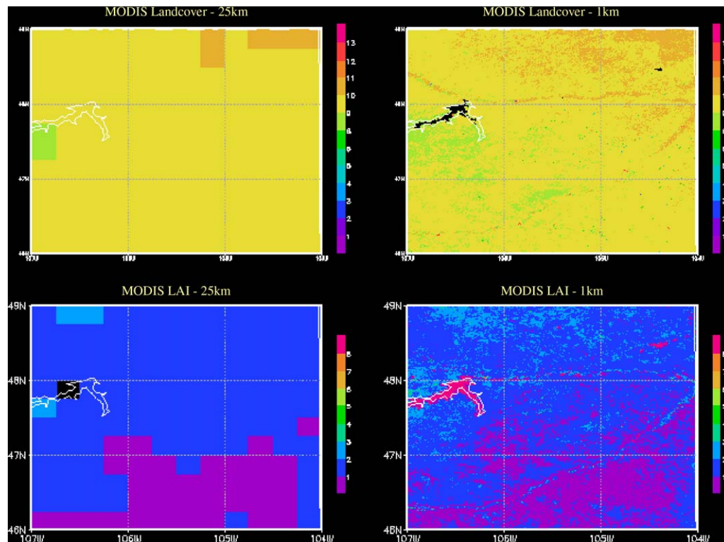
Fig. 10. Comparison of the 1 km and 25 km data sets for landcover and Leaf Area Index (LAI) from MODIS datasets for Fort Peck, MT.
