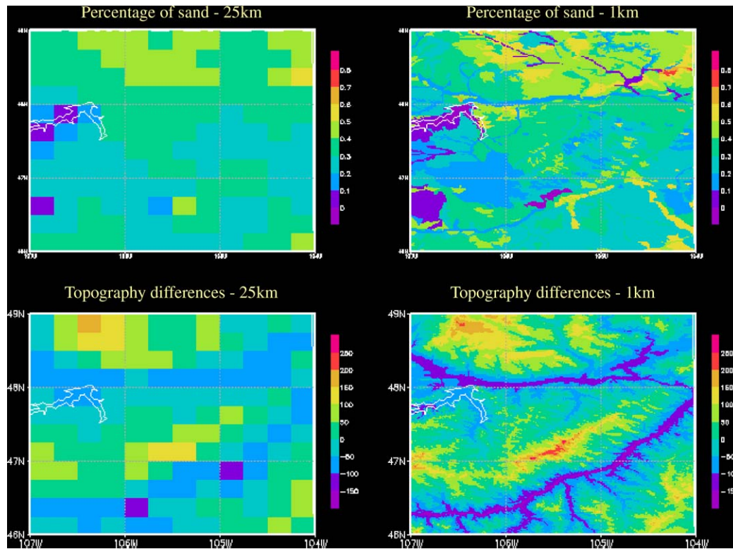
Fig. 9. Comparison of the 1 km and 25 km data sets for soil (sand fraction), and topography differences (between the 1 km topography and model) for Fort Peck, MT.
